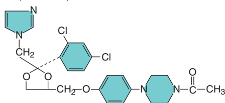
Ketoconazole (imidazole)
