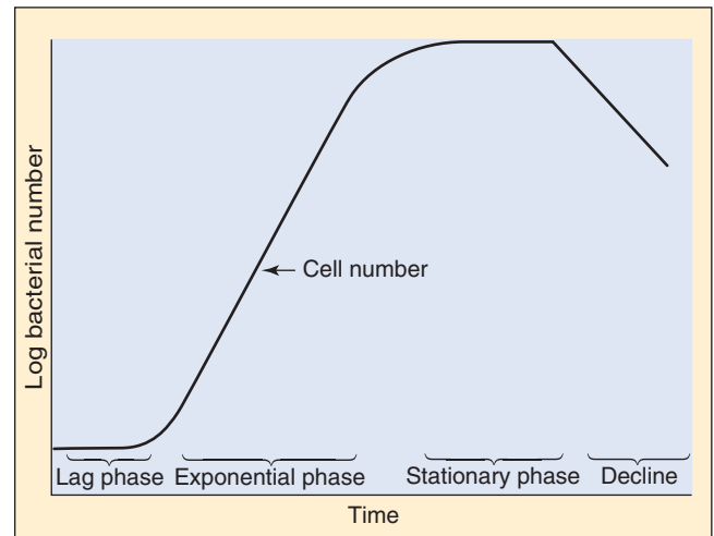
FIGURE 13-9 Phases of bacterial growth, starting with an inoculum of stationary-phase cells.
